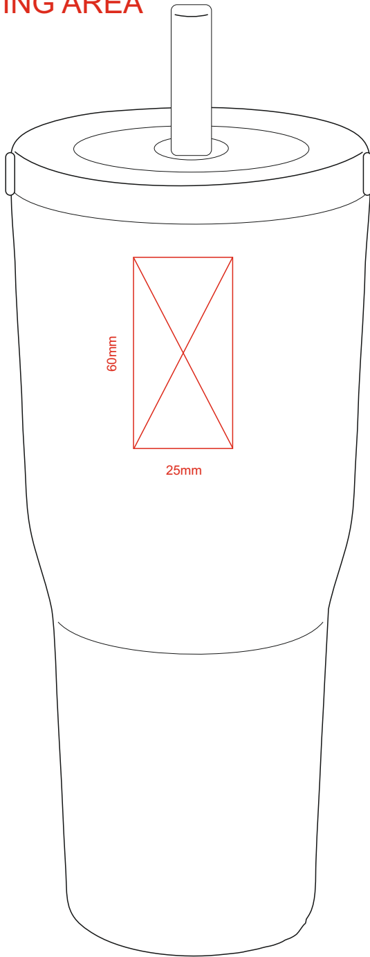
STANDARD ENGRAVING
